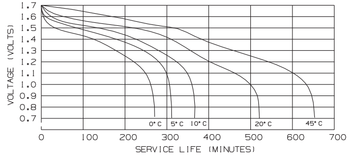
Discharge Characteristics 0.25 W Continuous to 0.9 end Volts
