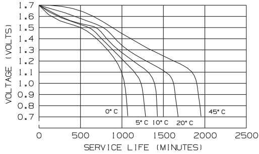
Discharge Characteristics 0.1 W Continuous to 0.9 end Volts
