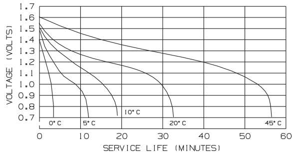
Discharge Characteristics 1.5 W Continuous to 0.9 end Volts
