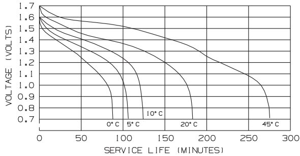
Discharge Characteristics 0.5 W Continuous to 0.9 end Volts
