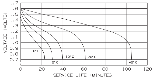
Discharge Characteristics 1.0 W Continuous to 0.9 end Volts
